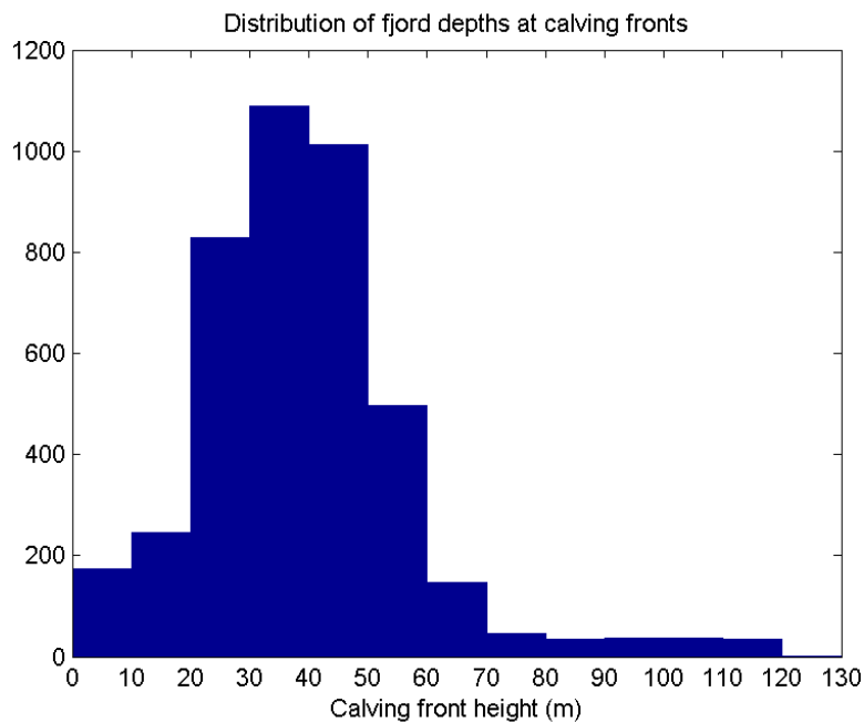
Figure 10 Distribution of measurements of fjord depth that are located within 500 m of tidewater glacier fronts. Dataset is geographically incomplete, but shows mean fjord depths is 40 m, with most fjords 50 m deep or less.
