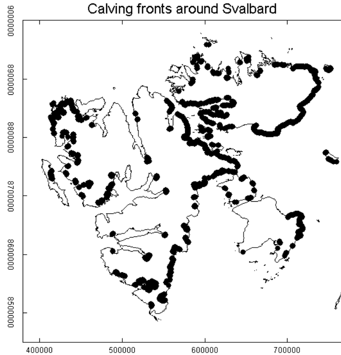
Figure 2 Distribution of glacier on Svalbard whose fronts lie in marine waters.
