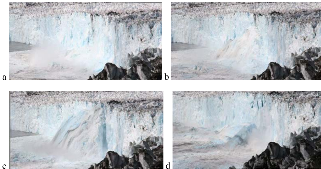
Figure 6 Submarine calving event at Columbia Glacier in Alaska. A large underwater ice block pops up and rotates on its side. To get a sense of the scale of the event, the exposed ice cliff height is about 120 m high (image from http://www.robfatland.net/seamonster/index.php?title=Columbia_Glacier_submarine_calving ).
