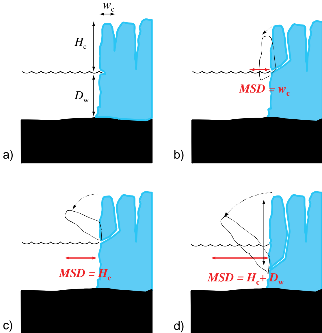
Figure 4 Calving processes: a) Calving front, with grounded crevassed ice feeding into fjord. Critical parameters are calving cliff height H_c , fjord depth D_w , and typical distance between crevasses w_c . Waves at the water line can erode and undercut the calving front. b) Calving event with failure at the water line, showing block gliding downward. Minimum safe distance (MSD) scales with w_c . c) Same as b), but with rotation outward. In this case, MSD scales with H_c . d) Calving event with failure occurring below the water line. In the extreme, a fracture plane may extend to the fjord bottom. In this case, MSD scales with H_c + D_w .
