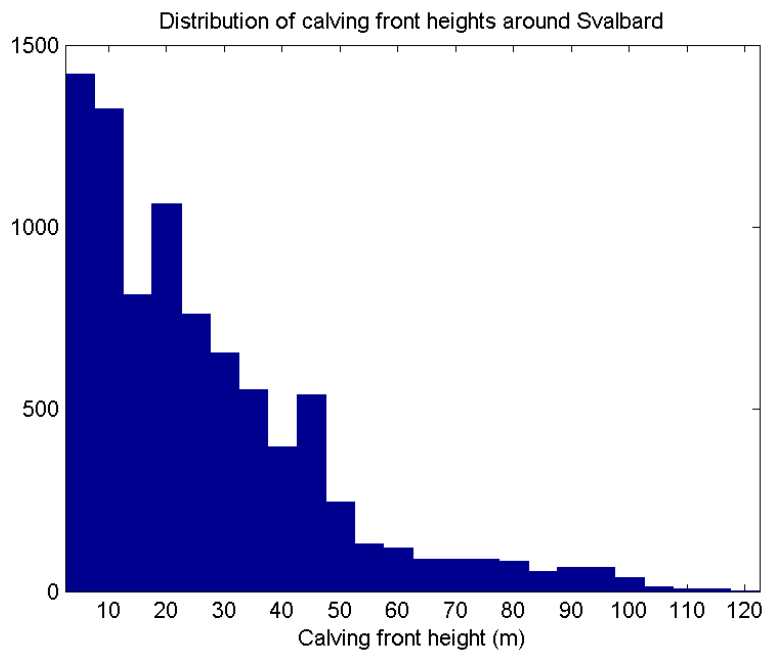
Figure 8 Distribution of exposed ice cliff heights shown in Figure 7. Many of the cliff heights over 60 m are incorrect, for reasons explained in the text.
