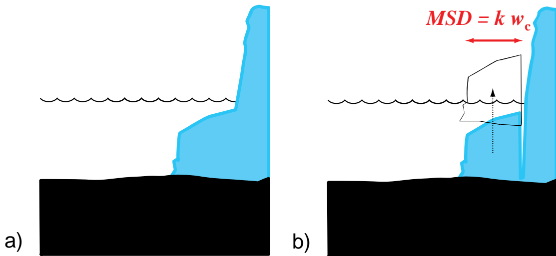
Figure 5 a) Ice foot below water line created after repeated calving above the water surface. b) Relatively short and thick ice foot, which will have a tendency to simply rise upward when it breaks. From the few observations available, a reasonable estimate of the foot dimension is some multiple of the crevasse width. However, some submarine blocks have been observed to surface at significantly greater distances from the ice cliff, so-called “shooters” (Table 1).
