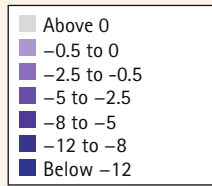
Permafrost temperature (°C) averaged for 1981–2000
