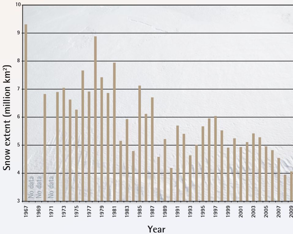
Summer Northern Hemisphere snow extent
