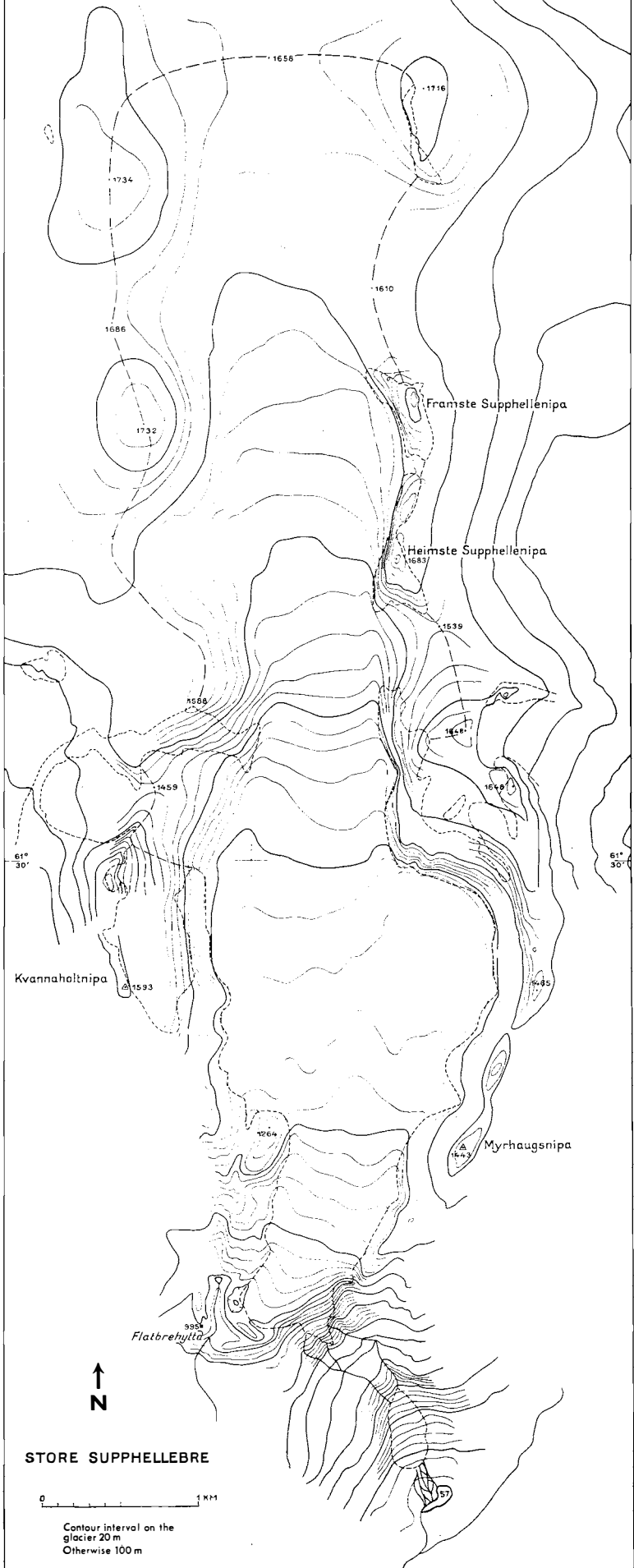
Fig. 3. Store Supphellebre. Based on 1:50 000 map constructed by the Cartographic Survey of Norway in 1967. Short dashes, ---, mark the glacier boundaries on land, long dashes, ---- mark the boundaries with adjacent snow fields and glaciers.
