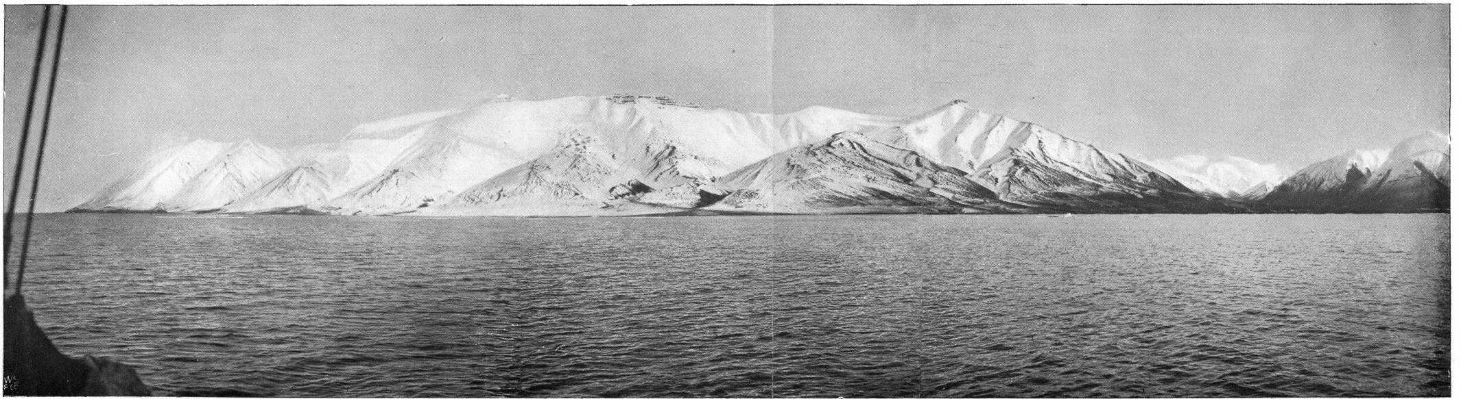
Fig. 1. East side of Wood Bay between Cape Auguste Viktoria and the Værdalen valley. Devonian sediments — to the left (N) Grey Hoek shale and sandstone, to the right Wood Bay sandstone — crowned by lavas (the high, white peak is Mt. Prisme fjell). G. Isachsen phot. Aug. 19. 1910. (From Isachsen).
