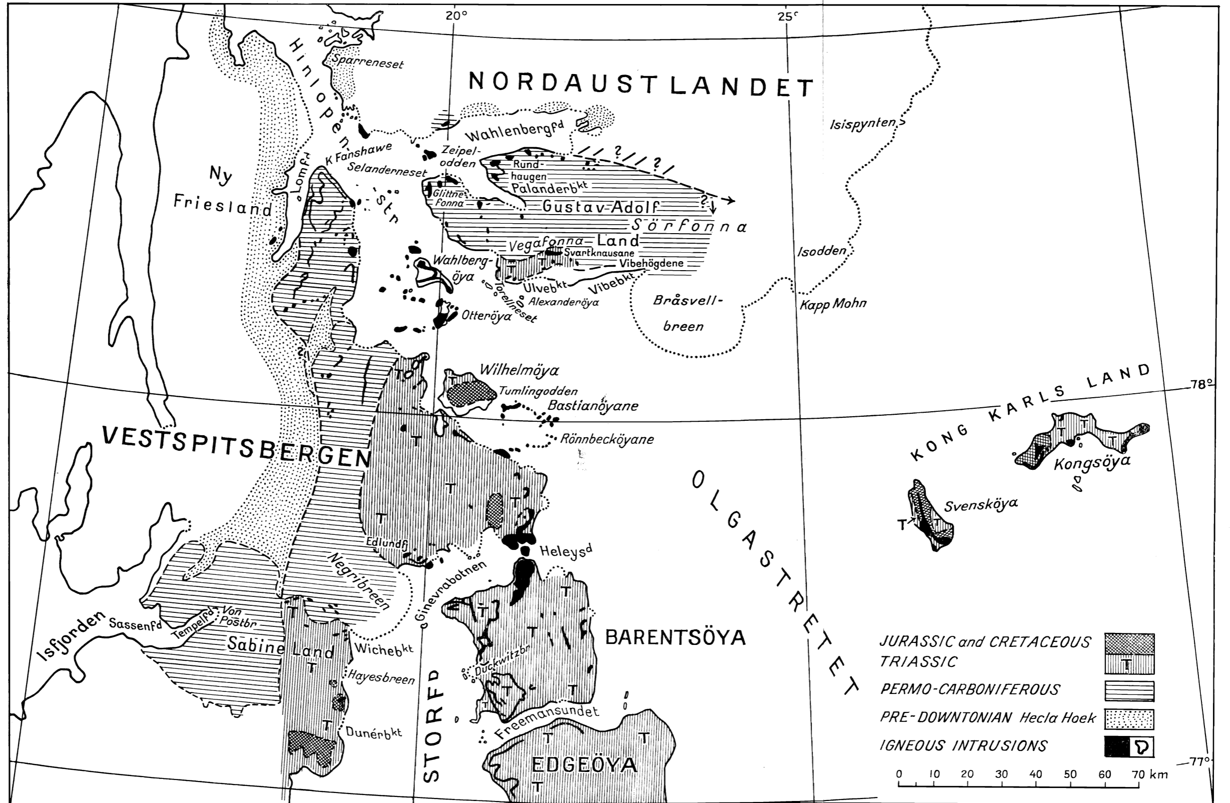
A geological sketch map of Hinlopenstretet and Northern Storfjorden by M. F. W. Holland
