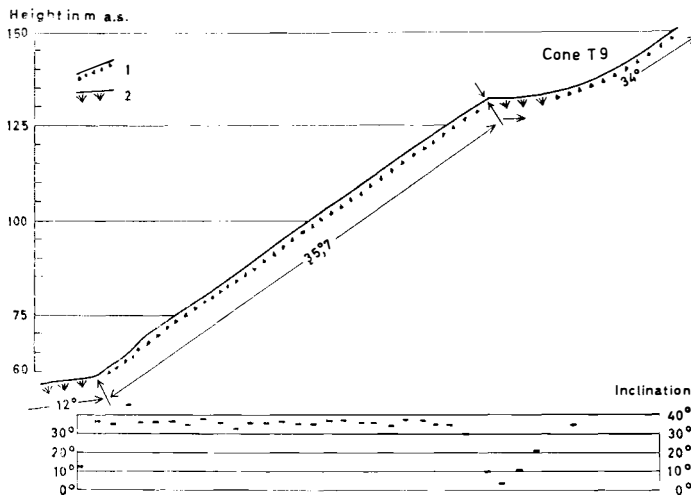
Fig. 15. Slope profile and inclination diagram from terrace at cone T9, Bjona-hamna (cf. Plate I). Horizontal scale same as vertical. 1, naked debris slope; 2, vegetation cover.
