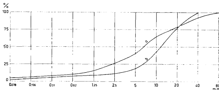
Fig. 14. Cumulative curves of particle-size distribution in relatively fine-grained material on talus cone T6, 100 m above sea-level. The material is probably from an old “mudflow levée”. The surrounding talus material was about 2–20 cm in size. a = surface, b = 0.2 m below surface.
