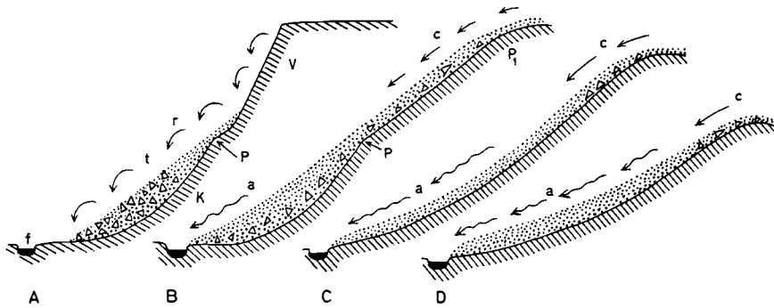
Fig. 2. Sketch showing the principles of slope development, modified by the author after Derruau (1956, p. 59); the later phases are according to the theories of Baulig and Birot.
