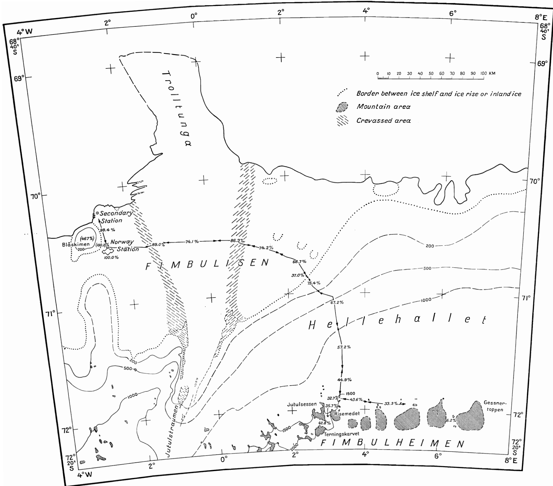
Fig 19. Accumulation in different parts of Dronning Maud Land as percentages of that at Norway Station. Values in brackets give only the summer-accumulation. Uncertain contours are stippled. Inset, the stake area at Norway Station. Altitudes in metres.
