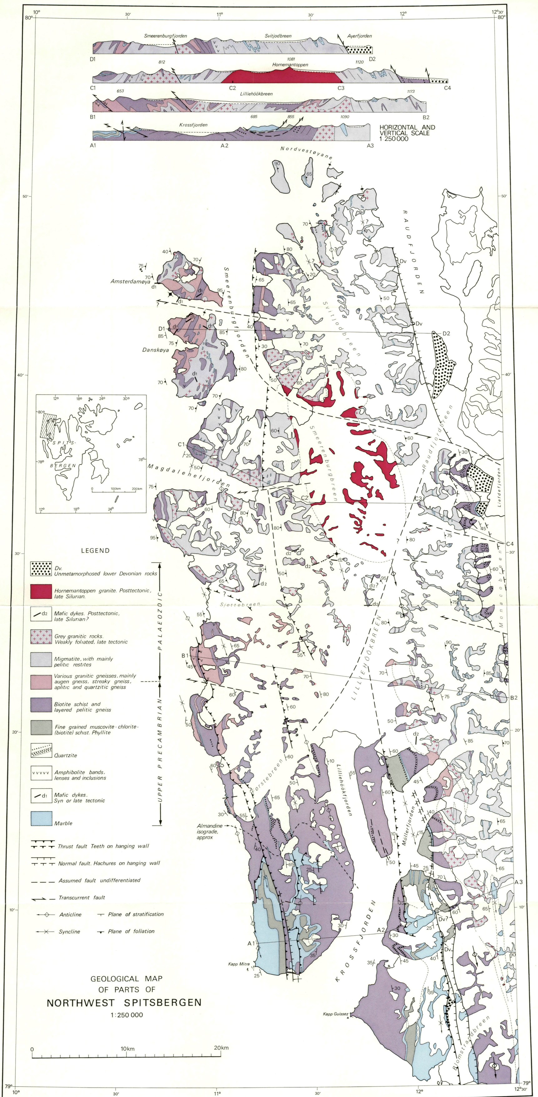
Fig. 9. Geological map of northwest Spitsbergen. Scale 1:250 000.
