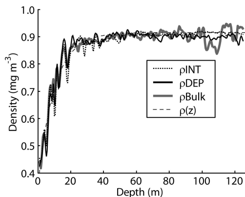
Fig. 5. The DEP, INT and weighed (Bulk) density records plotted versus depth, together with the expected density \rho(z) . For better visibility, the data have been smoothed using a Gauss filter with \sigma = 0.5 m. The thin dashed black curve is the calculated density \rho(z) using Equation (5).
