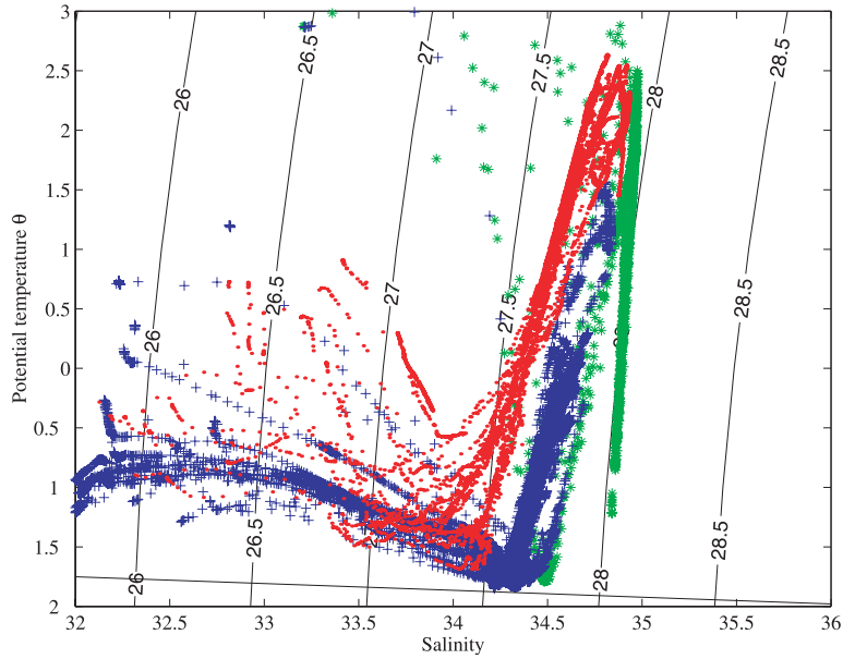
Fig. 4. \theta S diagram of all the CTD profiles from the transect. Green stars are observations in Hopen dyppet, south of Storbanken (south of 76.5^\circ N). Blue crosses are observations at Storbanken, from 76.5^\circ N to 79^\circ N. Red dots indicate the observations north of Storbanken (north of 79^\circ N).
