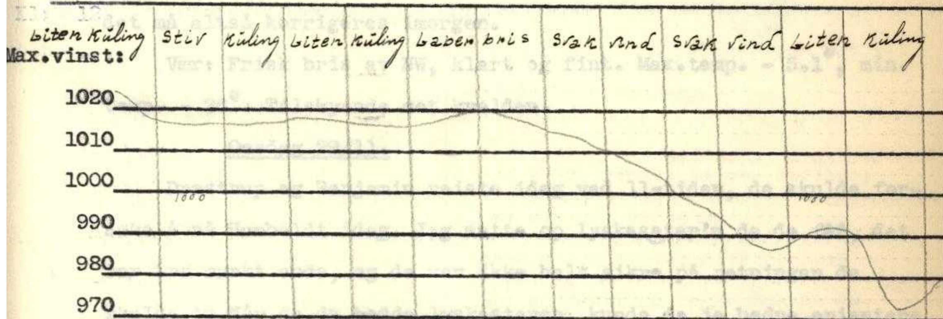
Barogram for uken 20/11 - 27/11 1933.
