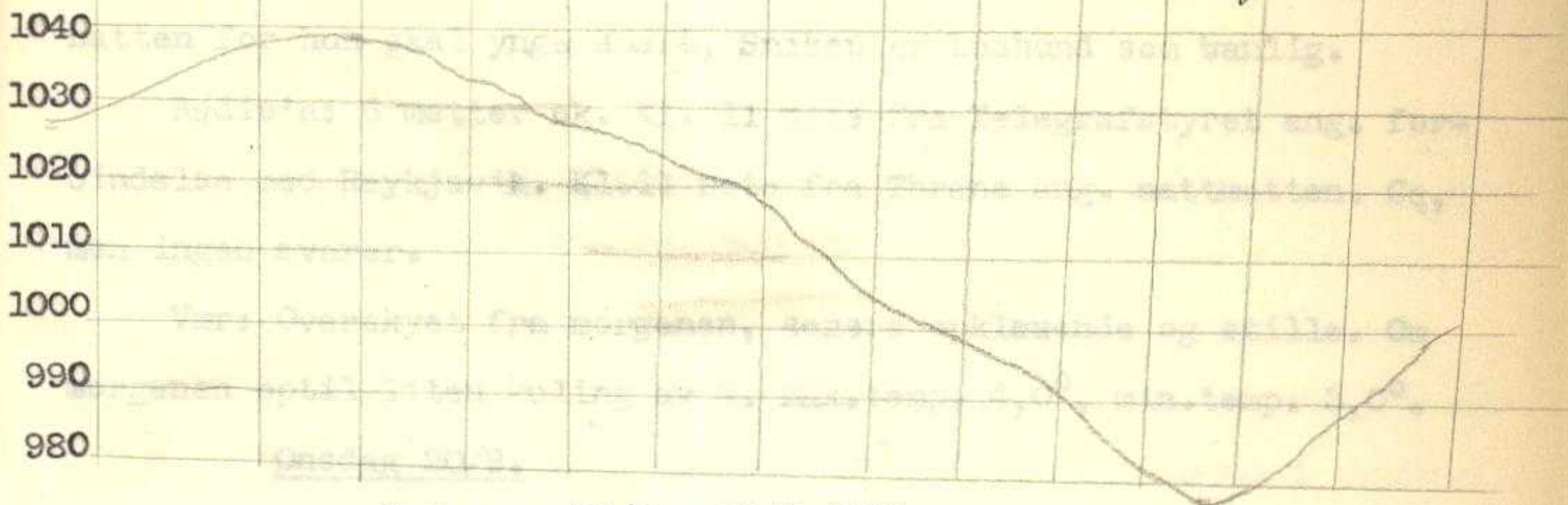
Barogram 11/9 - 18/9 1933.
