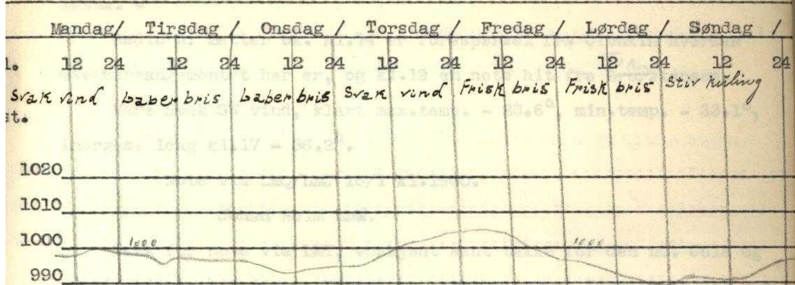
Barogram 8/1 - 15/1 - 1935.
