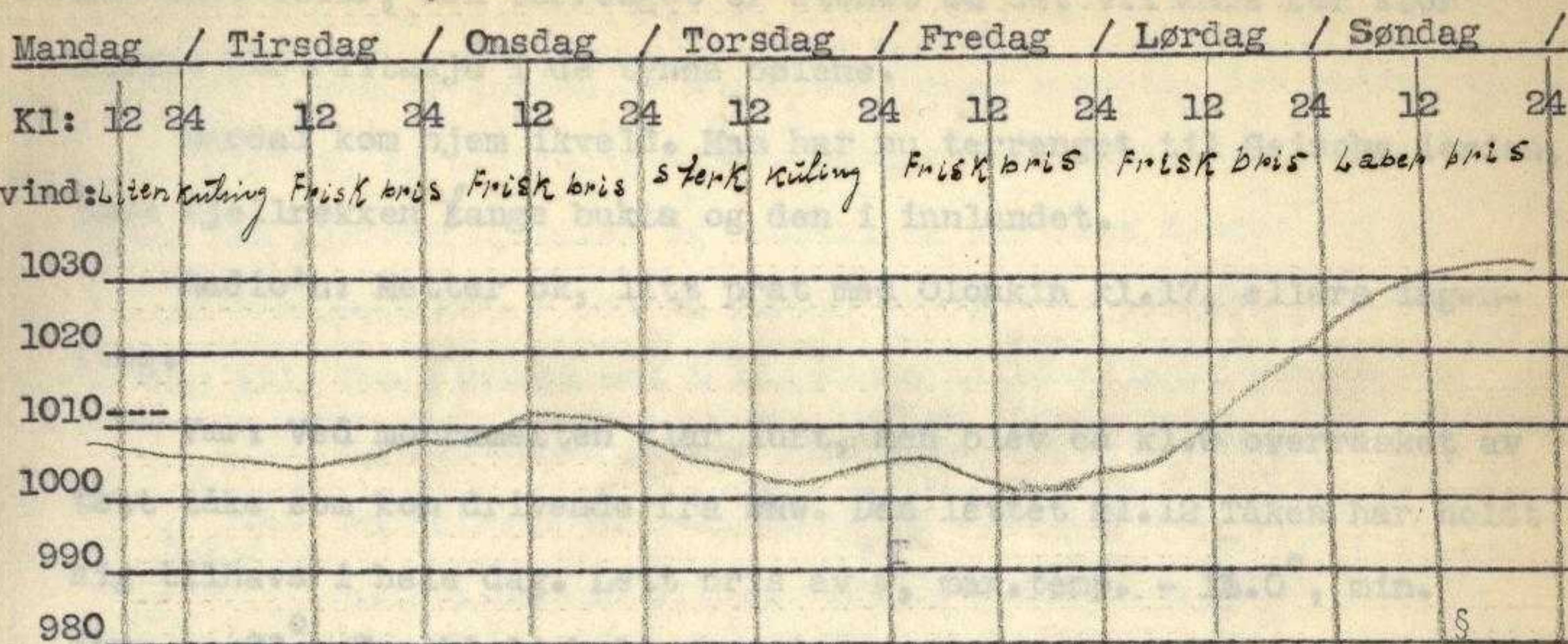
Barogram 16/10 - 23/10 1933.
