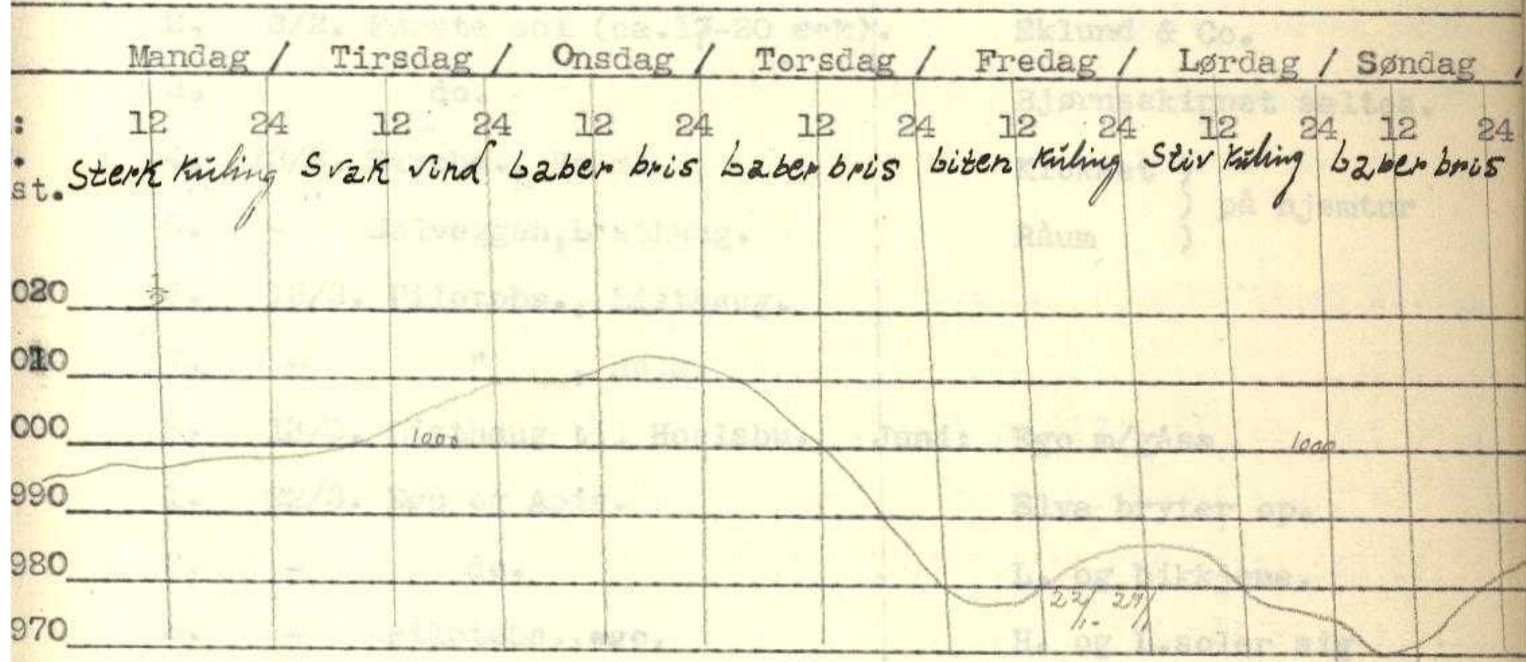
Barogram 22/1 - 29/1 1934.
