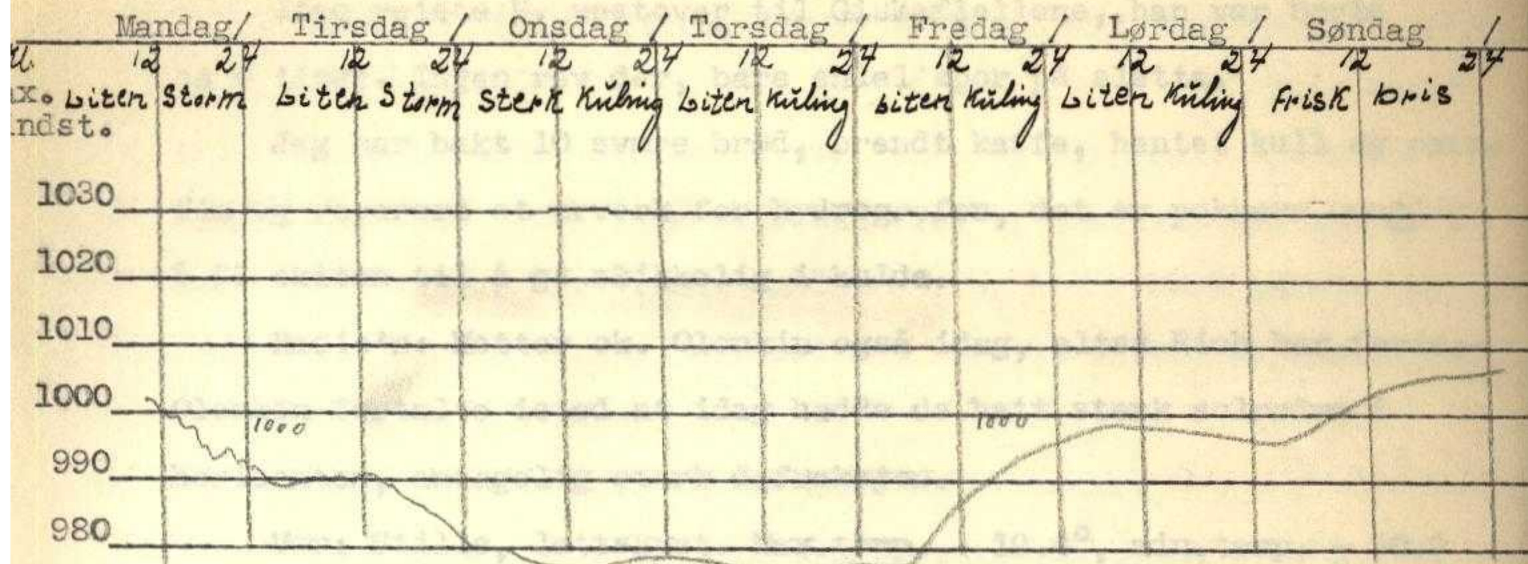
Barogram 1/1 - 8/1 - 1934.
