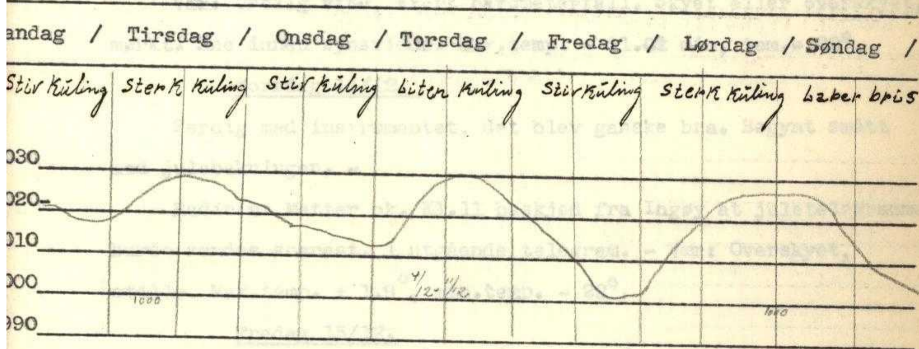
Barogram 4/12 - 11/12-1933.
