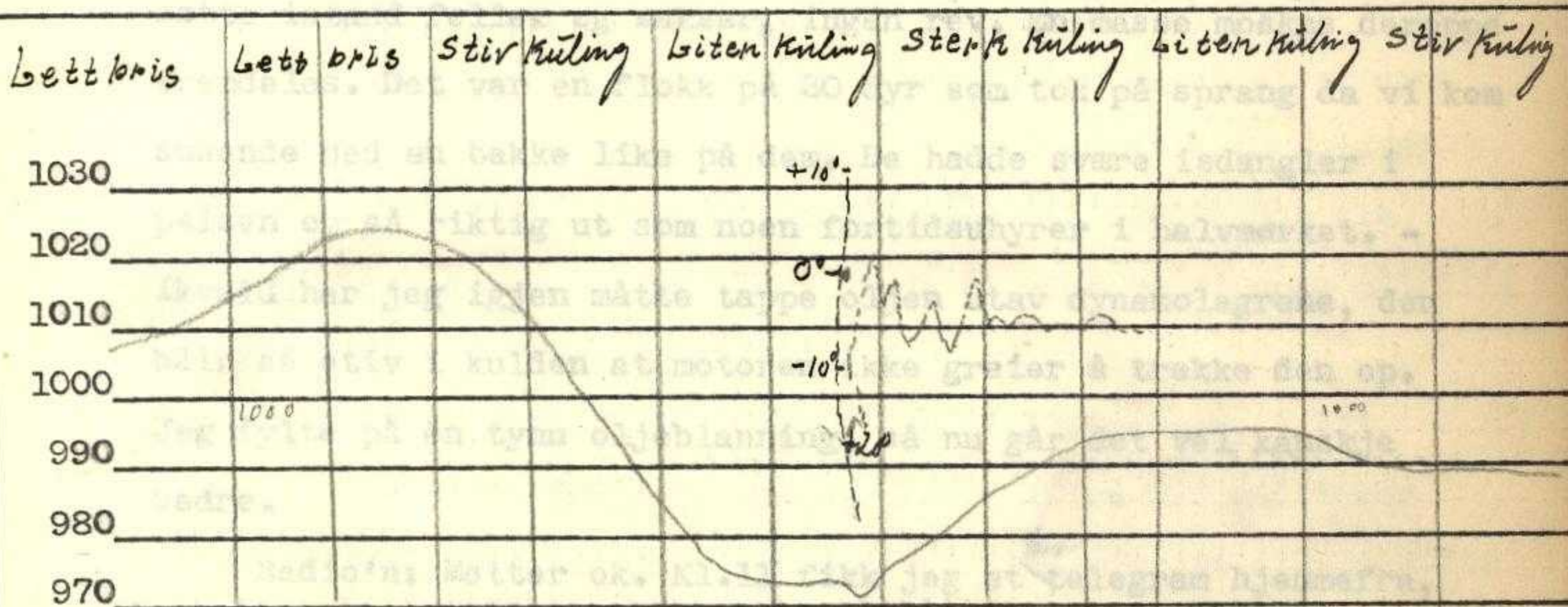
Barogram 11/12 _18/12 1933, m/Temperaturkurve 14/12.
