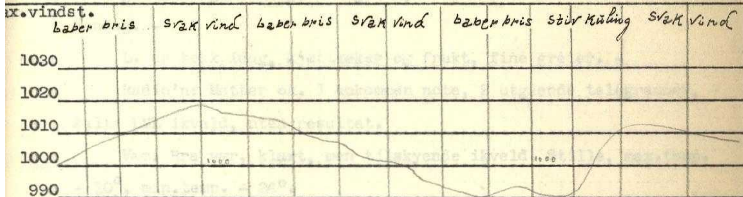
Barogram 18/12 - 25/12 1933.
