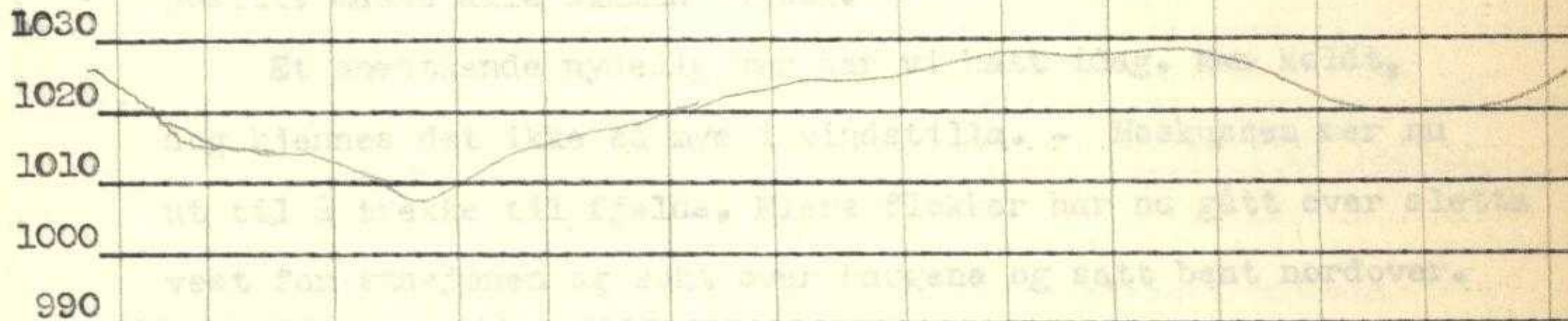
Barogram 2/10 - 9/10 1933.
