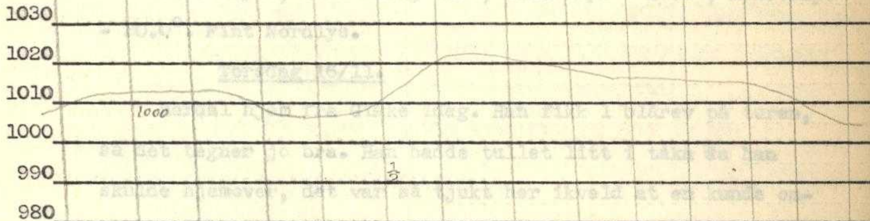
Barogram 6/11 - 13/11 1933.
