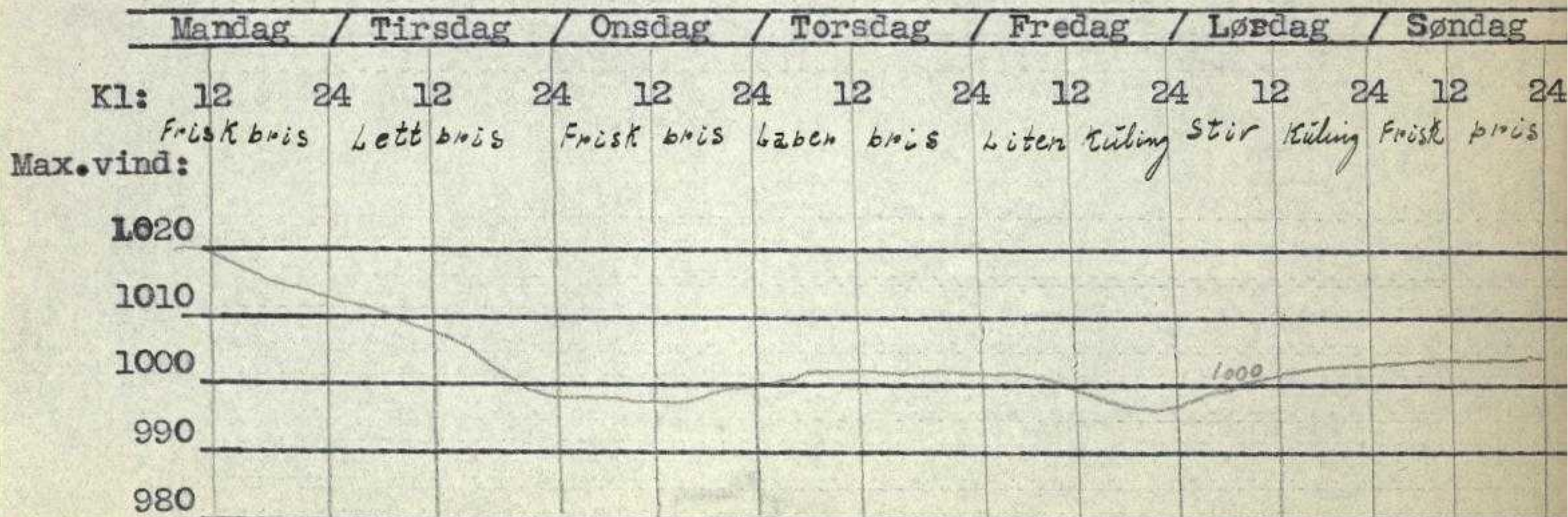
Barogram 9/10 - 16/10 1933.
