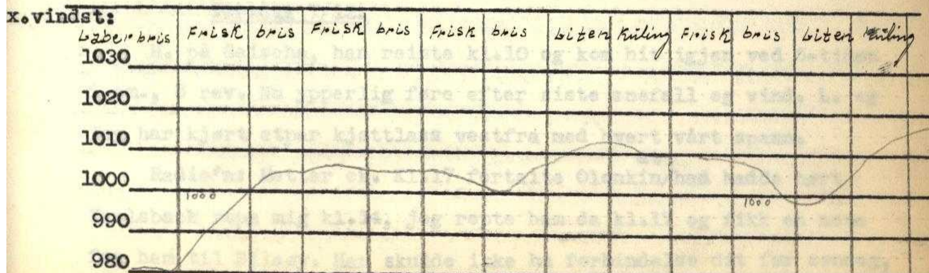
Barogram 27/11 - 4/12 1933.
