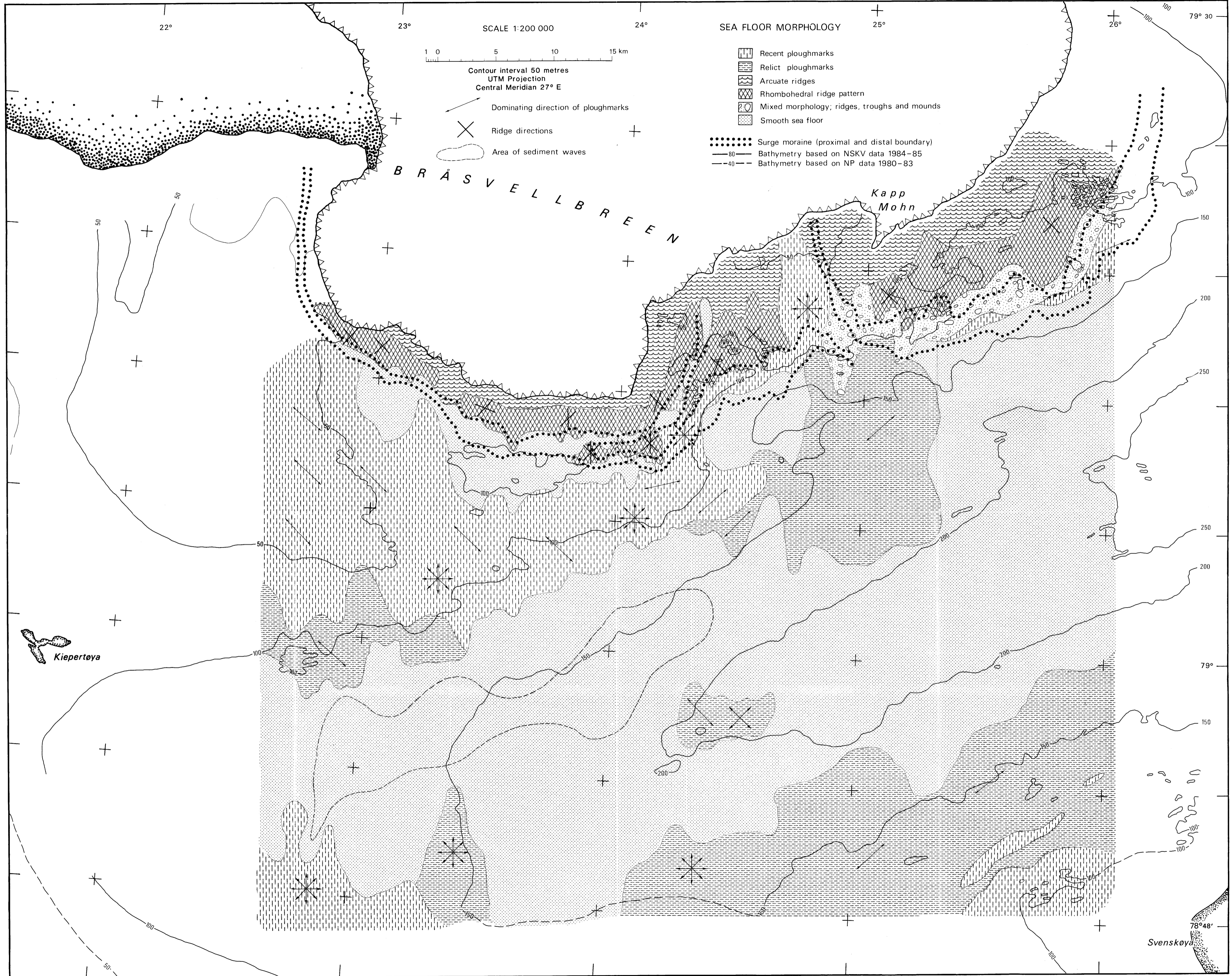
Fig. 7. Map showing morphological provinces. Each province is characterized by its dominating morphological pattern. (Paper 2; Solheim, A: The depositional environment of surging sub-polar tidewater glaciers.)
