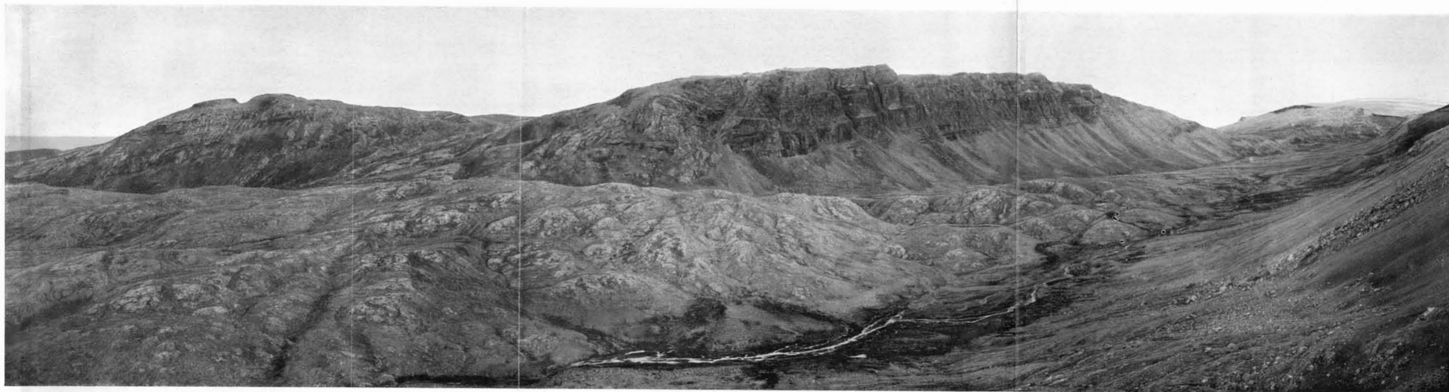
A. Ymesdalen seen from the northwest. The Tetradium Limestone makes up the hills in the valley and also Antarcticfjellet in the background.
