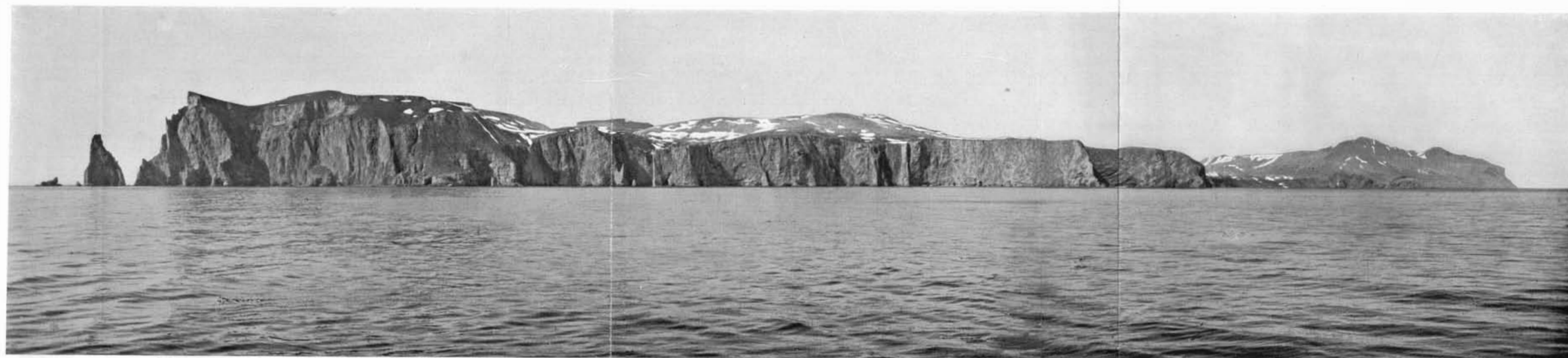
A. The coast from Fuglefjellet to Sørhamna. The cliff is made up of Younger Dolomite belonging to the Hecla Hoek. Fuglefjellet is capped by Carboniferous limestone. Miseryfjell in the background to the right.
