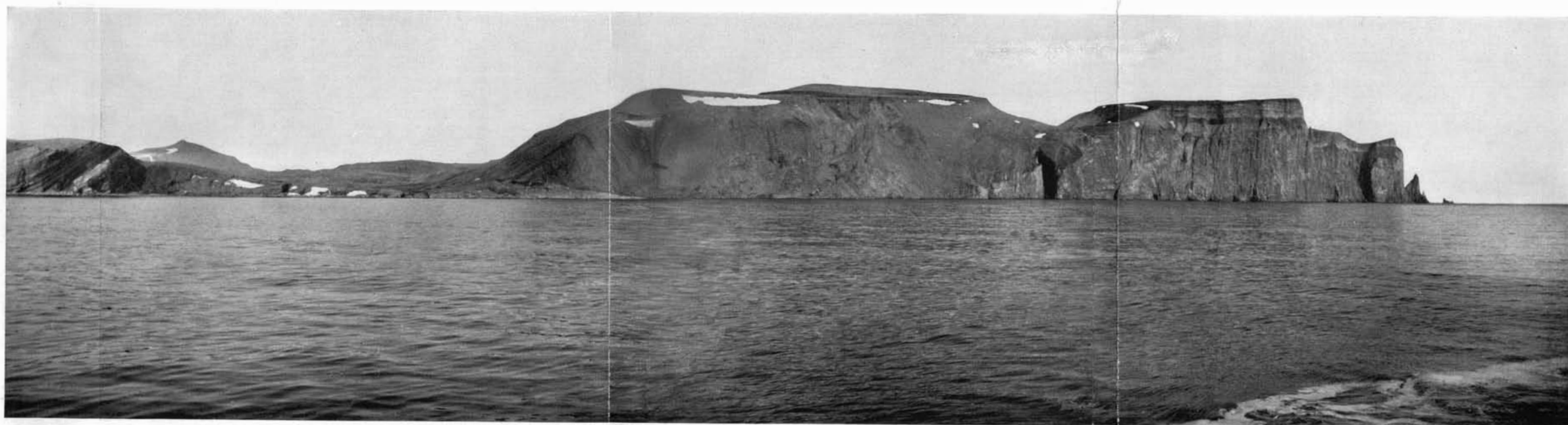
B. The southwest coast from Ellasjøen to Stappen.
