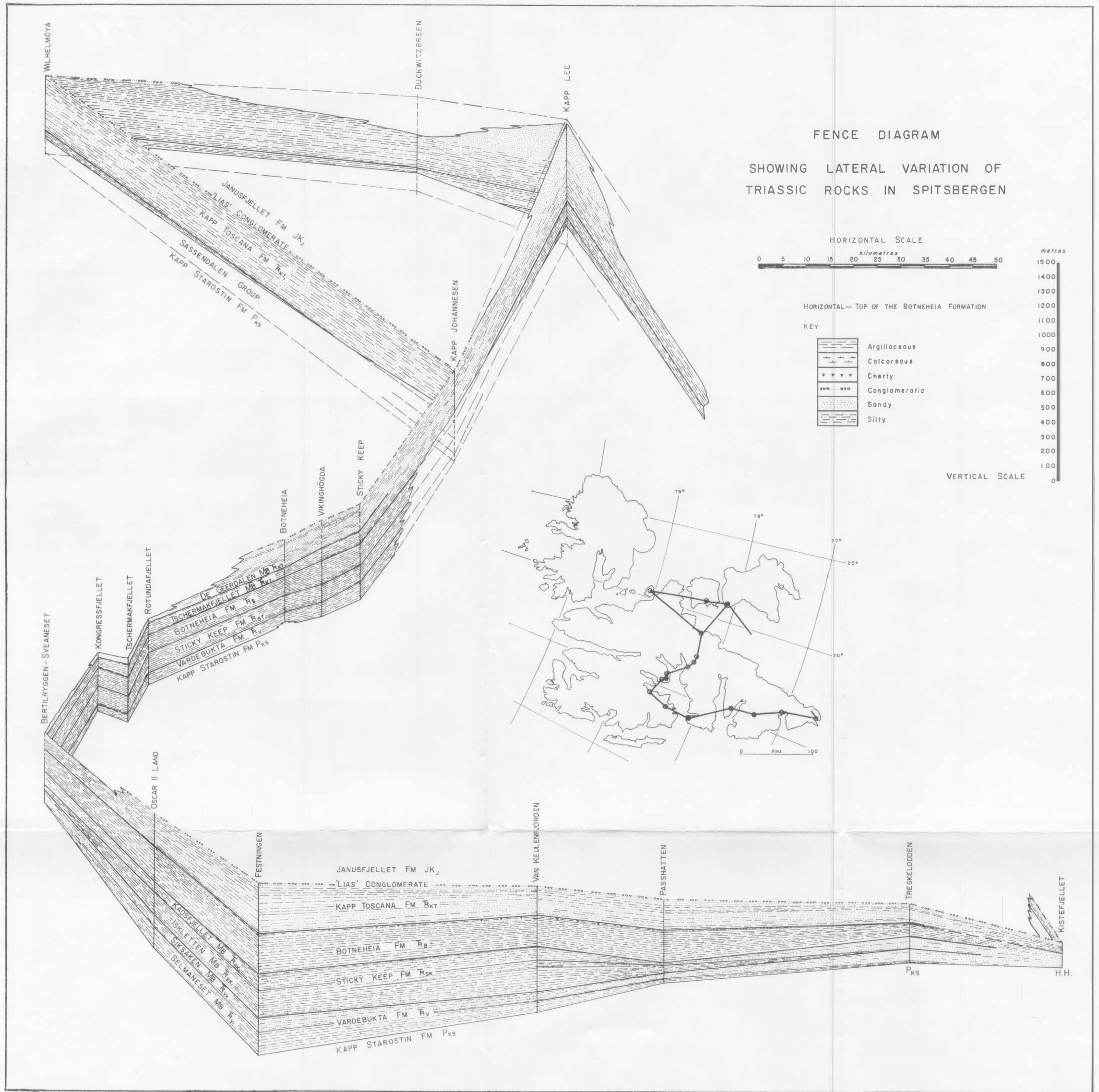
Fig. 25. Fence diagram showing lateral variation of Triassic rocks in Spitsbergen. This is based on the information given in figures 4 to 24 together with the outline Triassic succession for Edgeøya given in KLUBOV 1964.
