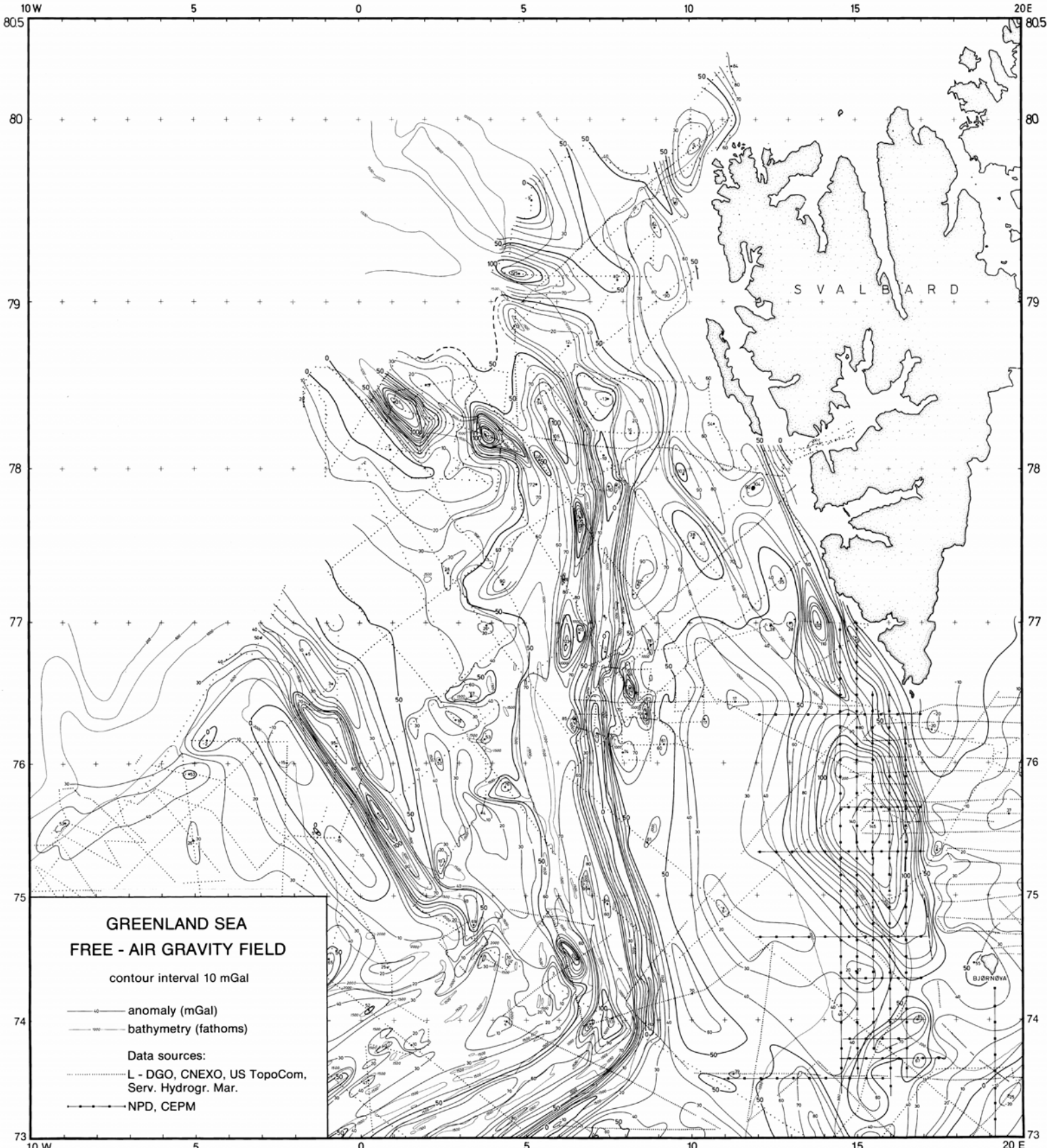
Fig. 2. Free-air gravity anomaly map of the Greenland Sea. Bathymetry from Talwani & Gorda (1976). Echelon Nord Polaire/Arctic Skanlon No. 180 (1981).
