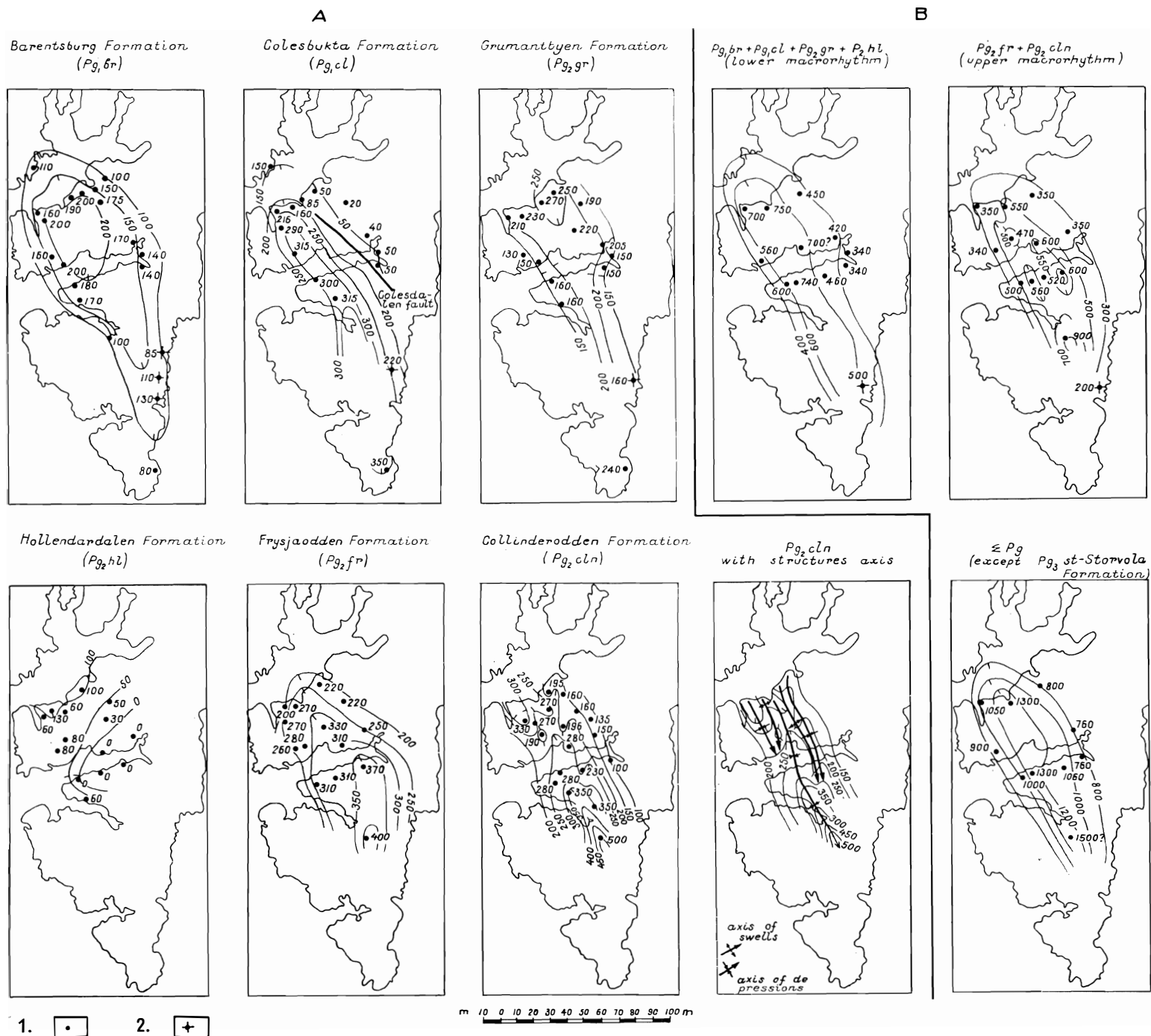
Fig. 3. Thicknesses of Palaeogene deposits in the Central Basin (Spitsbergen graben-like trough). A. Isopachytes per 50 m. B. Isopachytes per 200 m. Thickness values are given: 1. based on the author's data (on the south-eastern coast of Van Mijenfjorden after A. I. PANOV and V. F. NEPOMILUEV, unpublished data); 2. after NAGY (1966).
