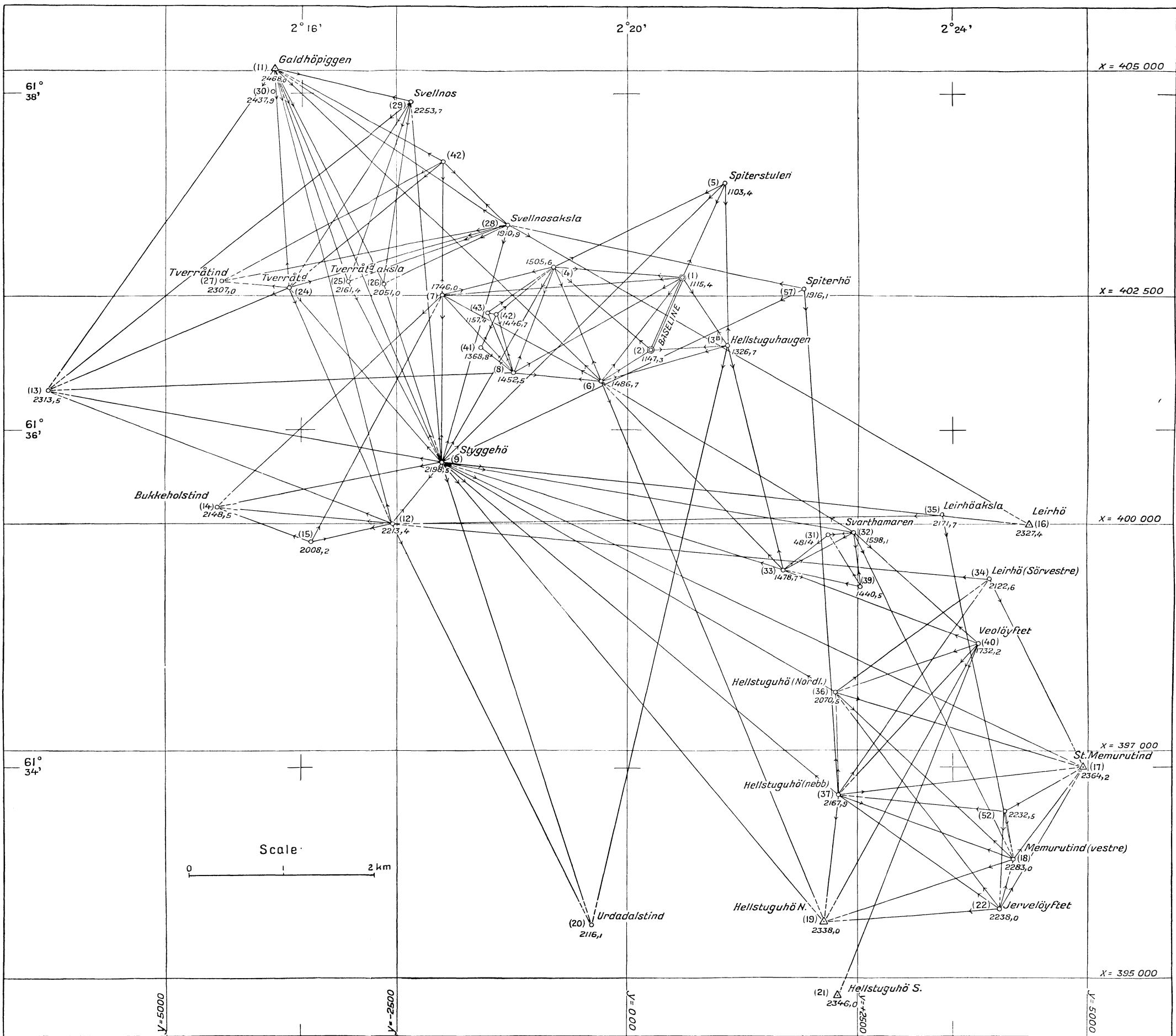
Fig. 92. The trigonometrical net used for the survey of Hellstugubreen, Svellnosbreen and Tverråbreen.
